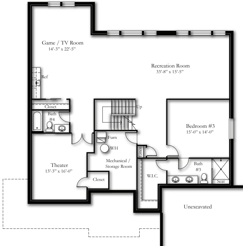
Option III Finish Basement Floor 1,926 Sq. Ft.
