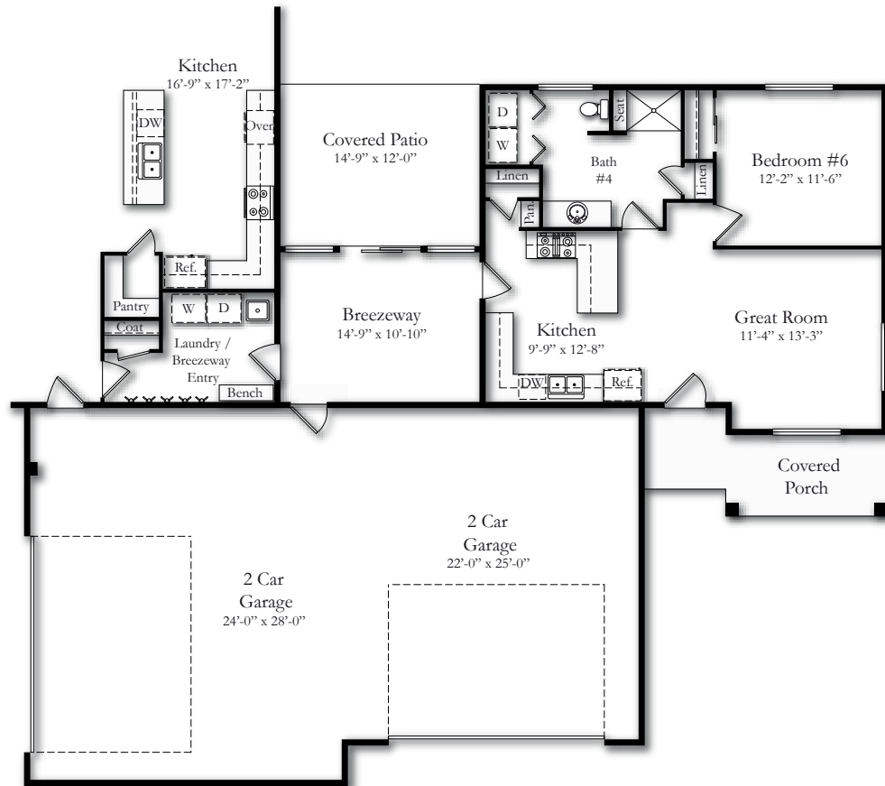
Opt. ADU Main Floor Without Basement 750 Sq. Ft.
